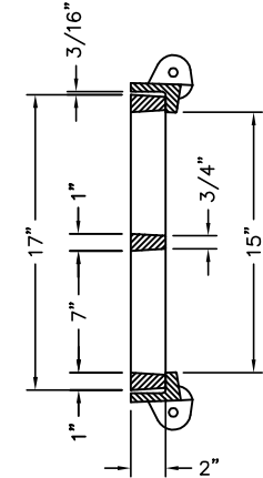
R-4990-EA TYPE "A" GRATE AND TYPE "X" FRAME
