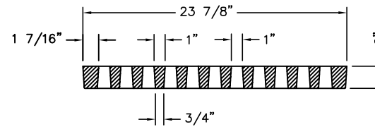
SECTION THRU GRATE
