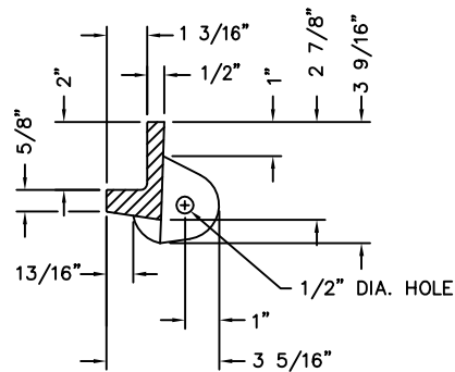
SECTION VIEW SCALE 1:4
